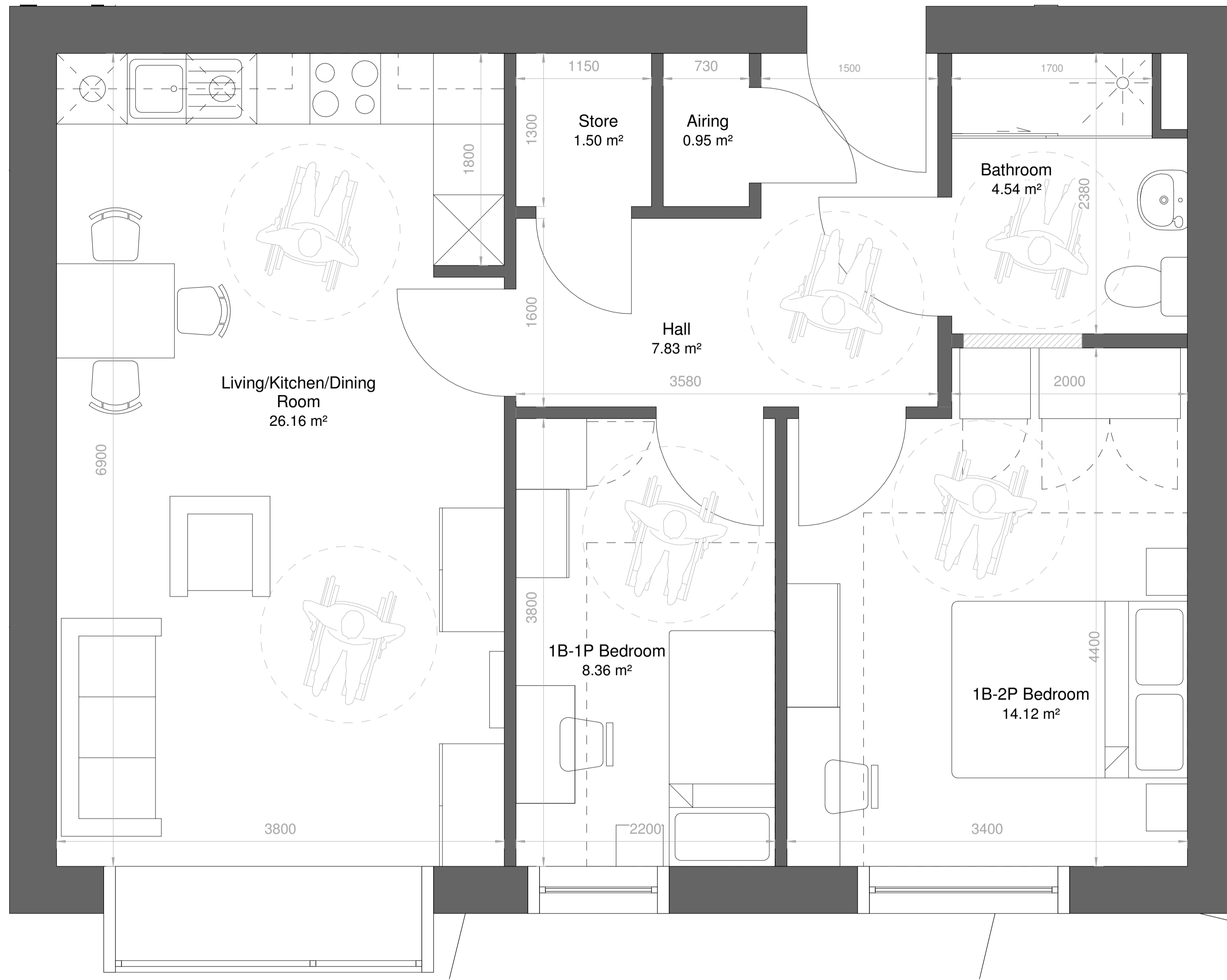
2Bed Apartment Area: 66 Sqm 1 : 25
