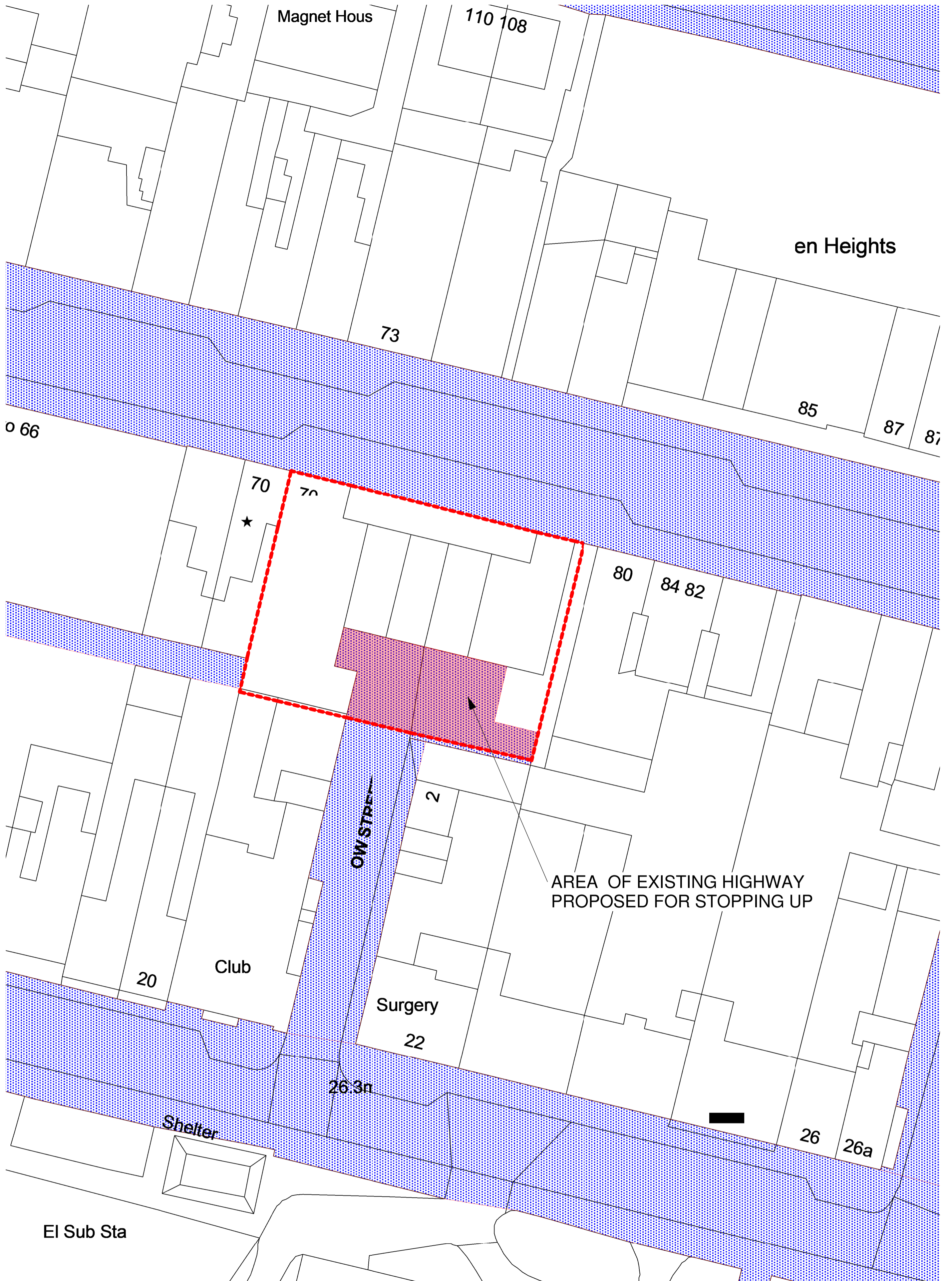
Proposed stopping up plan of vehicle turning head within site. 1 : 200
